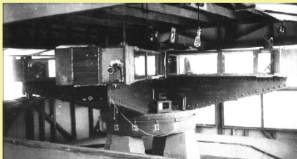
Dayton Miller's Ether-Drift Interferometer, p.114, 131 & 137
